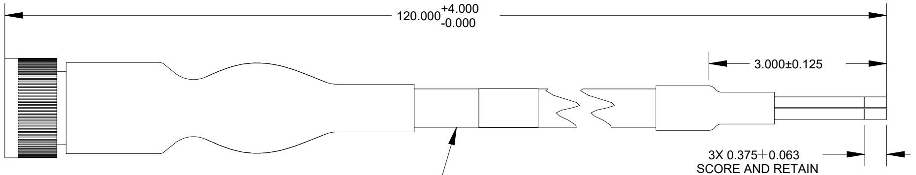
8 AWG WIRE WITH 3 CONDUCTORS (8/3) OVERALL NOMINAL WIRE DIAMETER:0.7"
