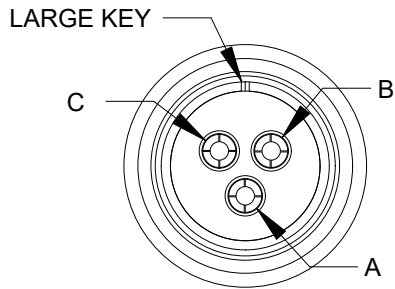
SOCKETS SCALE 0.750
